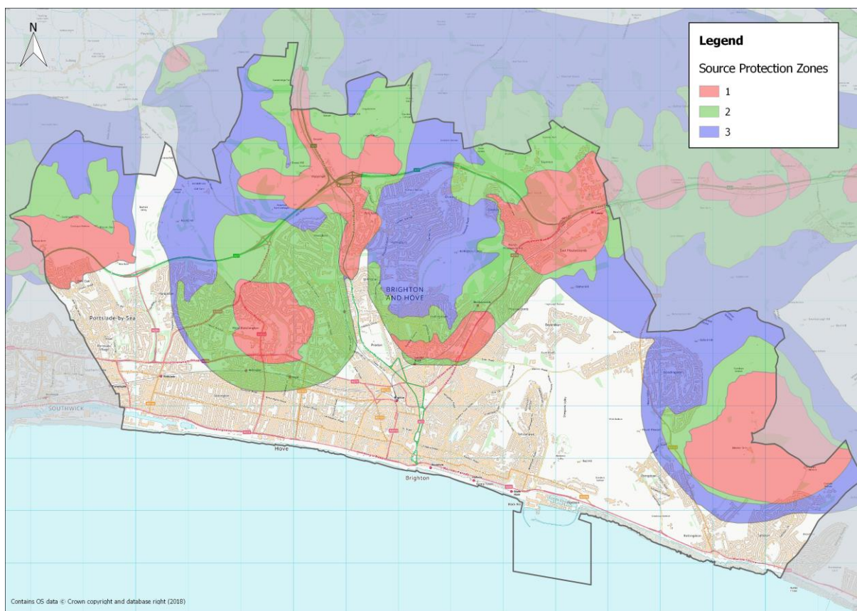
Figure 3. Ground water source protection zones
